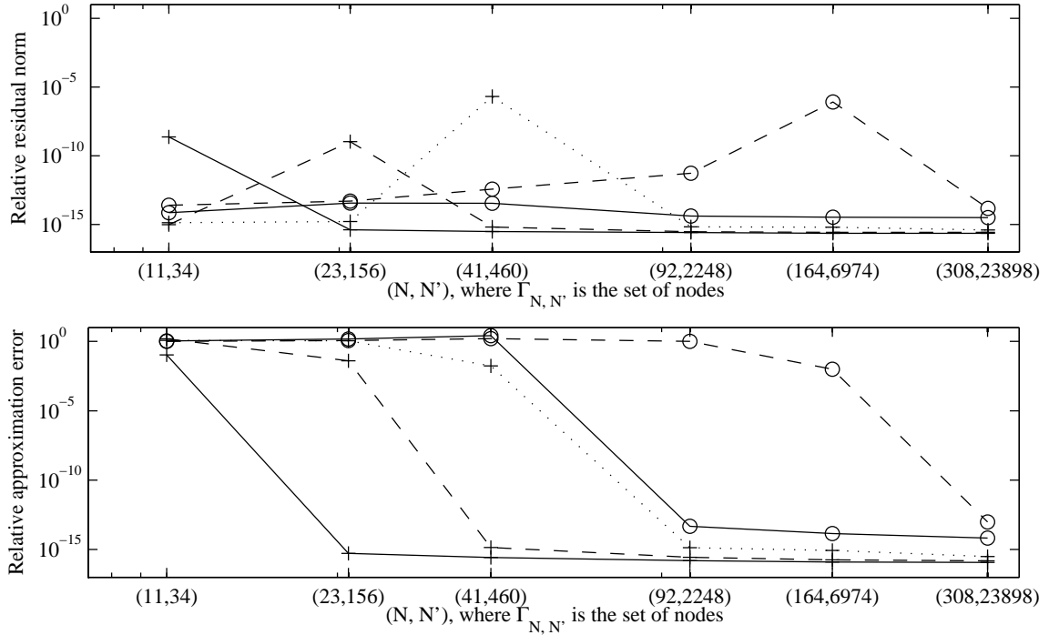
Figure 4.1: The relative residual norm \|\mathbf{P} - \mathbf{F}_{L,\Gamma} \mathbf{w}^R\|_2 / \|\mathbf{P}\|_2 in L^2(\text{SO}(3)) and the relative approximation error \|f - \mathcal{F}_{\text{SO}(3)} \mathcal{M} \mathbf{w}^R\|_{L^2(\text{SO}(3))} / \|f\|_{L^2(\text{SO}(3))} in L^2(\text{SO}(3)) of the CGNR based algorithms for polynomial degrees L = 5 (—+—), L = 10 (- -+ -), L = 20 (···+···), L = 40 (—○—), L = 80 (- -○ -). The dimensions |J_L| \in \{286, 1771, 12341, 91881, 708561\} compares to the cardinalities |\Gamma_{N,N'}| \in \{374, 3588, 18860, 206816, 1143736, 7360584\} of the sets of nodes.
